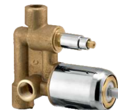
DB-1005 Divertor Body 40mm
